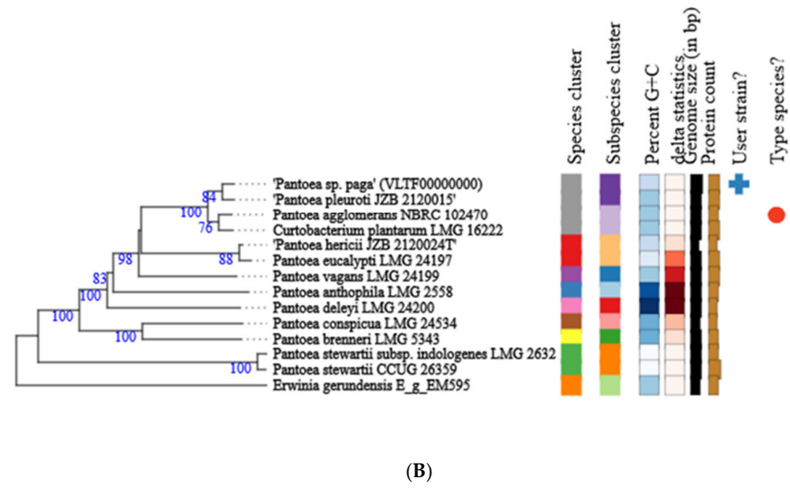
Figure 5. Phylogenetic tree of Pantoea paga strain calculated from 16S rDNA gene sequences (A); phylogenetic tree of Pantoea paga strain calculated from whole genome sequences (B). Different colors within each column indicate different minimum, maximum and intermediate values; + represents user strain and red dot indicates type species.
